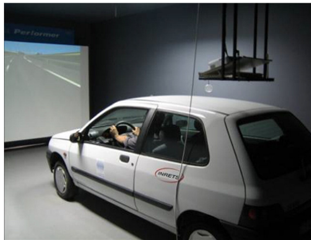
Fig. 1. Photography of the driving simulator.
